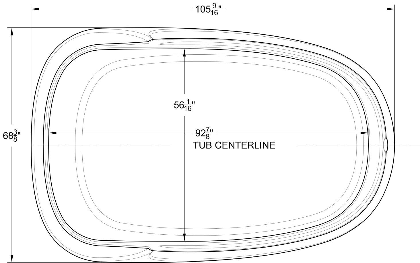
TUB BASE PLAN-VIEW (LID NOT OMITTED FOR CLARITY)
